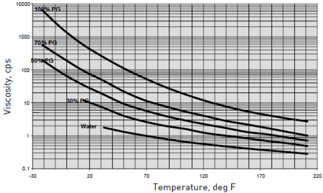
Viscosity of Aqueous Propylene Glycol Solutions
